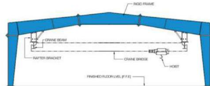
UNDERHUNG CRANE
