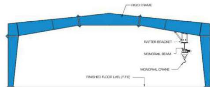
MONORAIL CRANE
