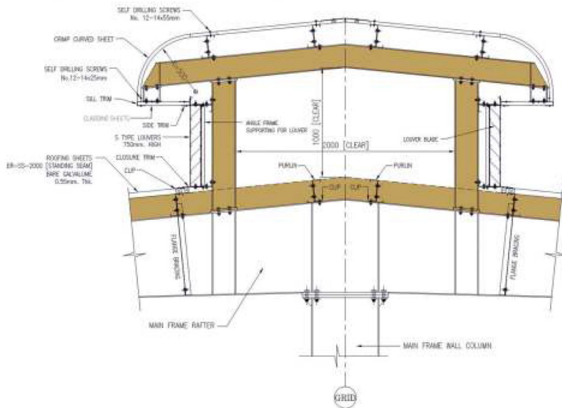
Roof Monitor
