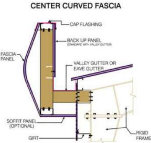
Fascia
