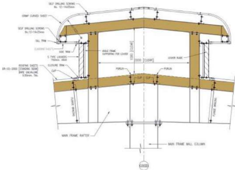
Roof Monitor
