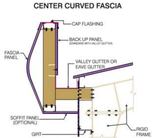
Fascia
